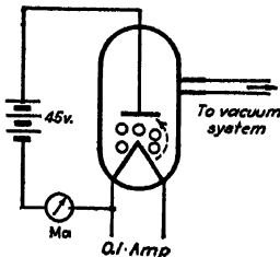
Circuit illustrating an emission-type ionization gage.
